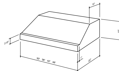
Installation height above the cooking surface: 24"-30"
